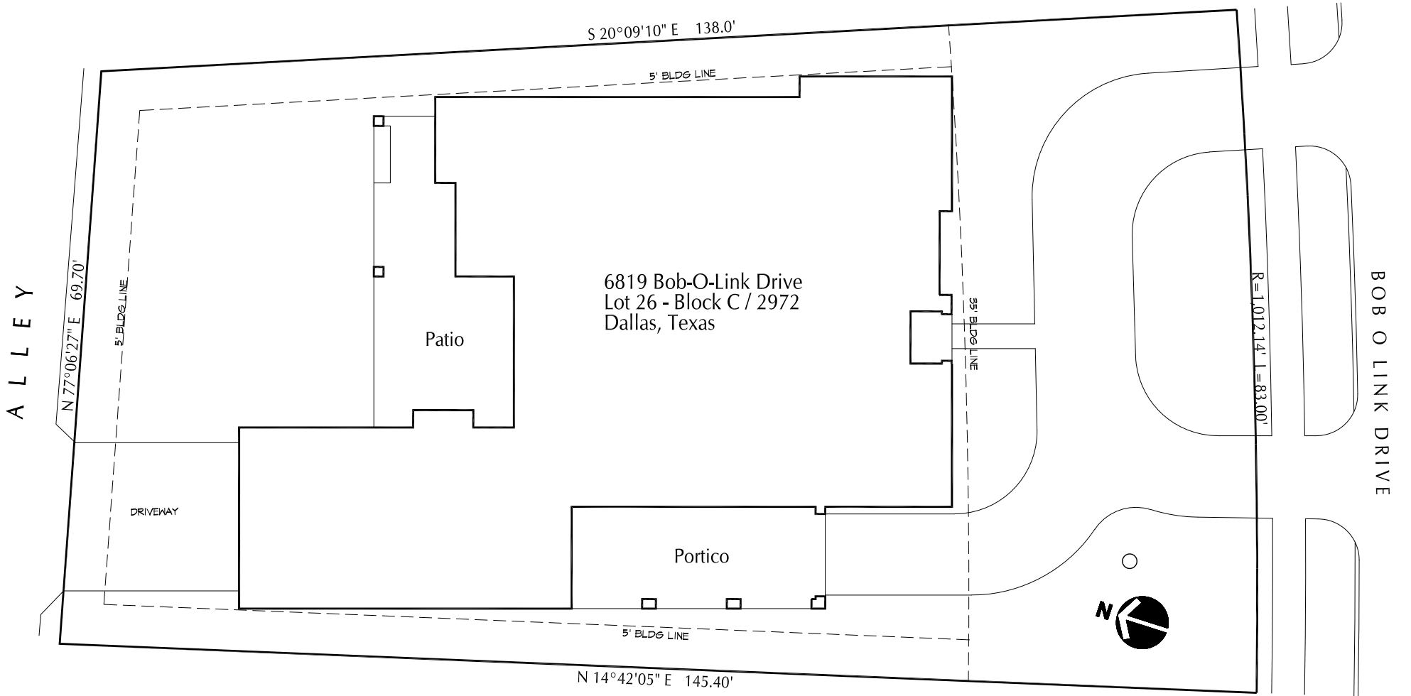
Site Plan 6819 Bob O Link Drive Dallas, Texas
